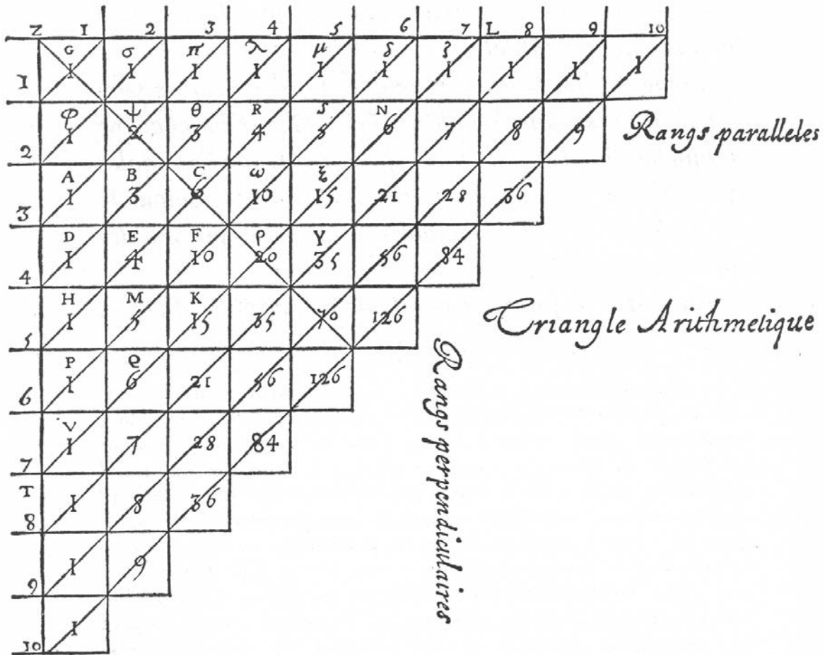
Figure 4: Pascal's arithmetical triangle
